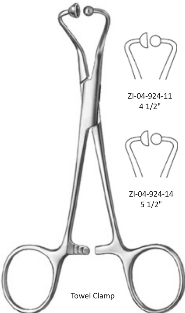
Towel Clamp Tohoku
