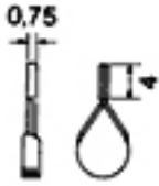
Mini Vessel Clip ZI-04-102-04 jaw 4,0 x 0,75 mmclosing pressure 60 gr.
