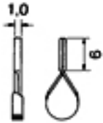
Mini Vessel Clip ZI-04-102-06 jaw 6,0 x 1,0 mmclosing pressure 85 gr.
